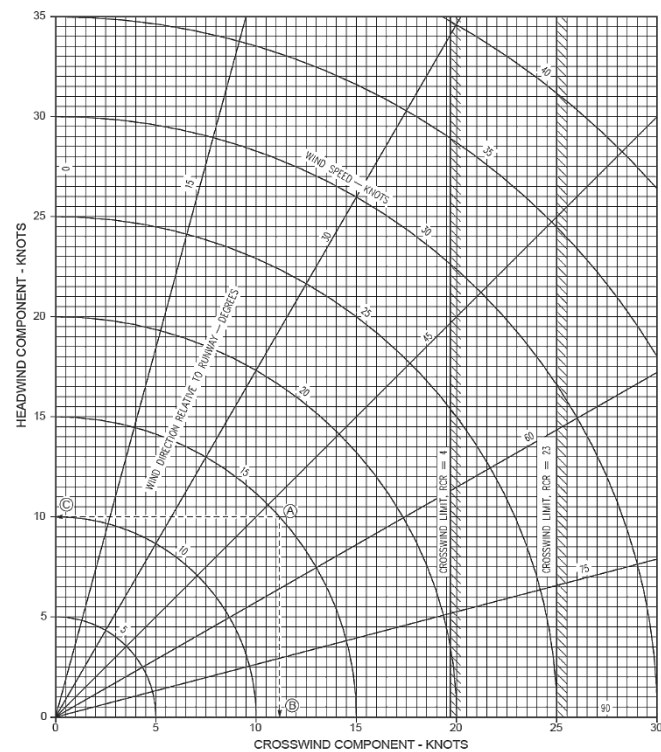
Figure N-2. Takeoff and Landing Crosswind Limits
